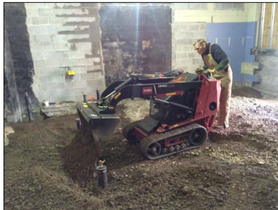
Backfilling, Restoring to Subgrade, and Compacting
